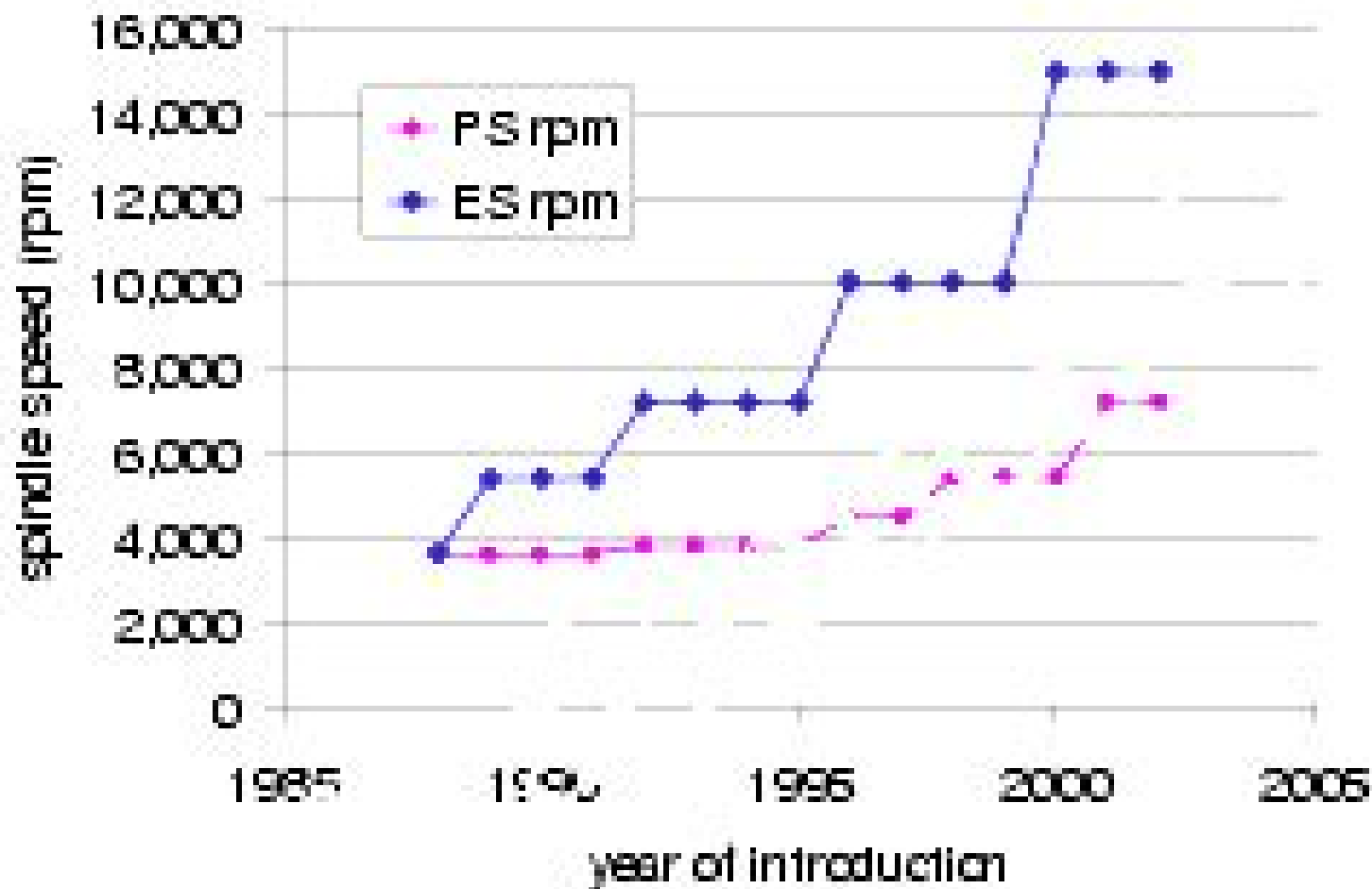
Figure 1: The adoption of higher rotational speeds. Data from Control Data product guides, 1988-1989 and Seagate product guides, 1990-2002.
